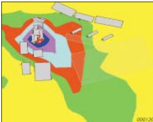
Noise contour map of an industrial complex
